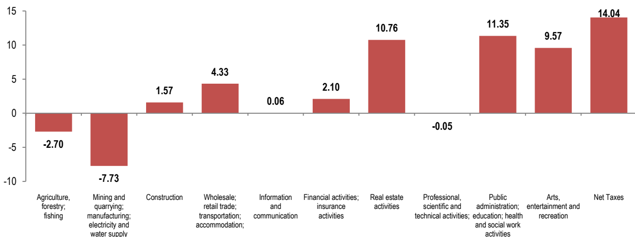
Fig. 2 Changes in % to the same quarter of 2023 for the main branches of the economy, (Q4_2024/ Q4_2023)
