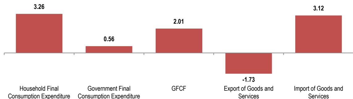
Fig. 3 Main components of GDP by expenditure approach, seasonally unadjusted (Q4_2024 / Q4_2023)%
