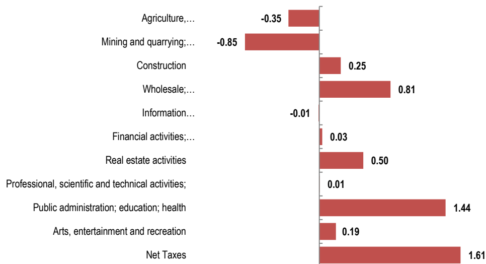
Fig. 1 Contribution of the main branches of the economy to real growth rate of GDP (Q4_2024/Q4_2023), in percent points
