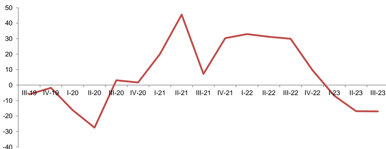
Fig. 2 Annual changes in Turnover volume index, Water supply; Sewerage, Waste management and Remediation activities (%)
